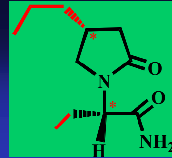
Brivaracetam
